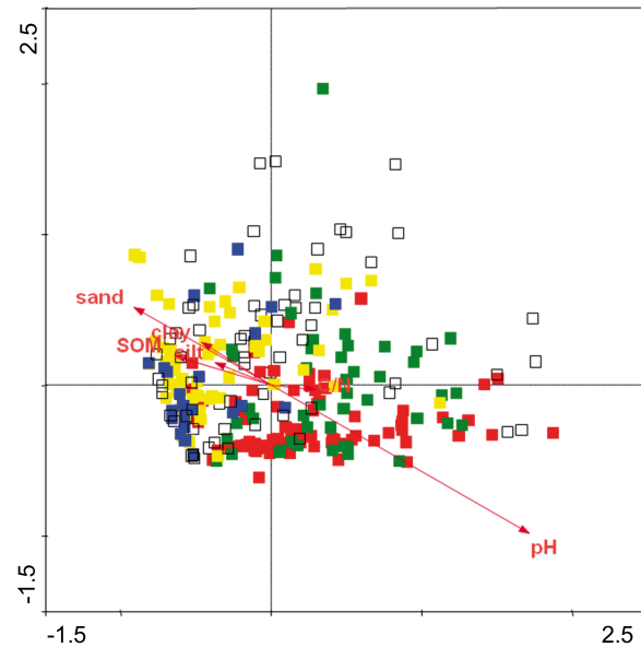
Figure 7. Principal component analysis based on abundance of 28 earthworm taxa determined to species level. Red – habitat type 33 (crop sites), green – 34 (grassland sites), yellow – 43 (deciduous forest sites), blue – 44 (coniferous forest sites), white – other habitat types. Length of gradient from detrended correspondence analysis = 3.3, first axis = 33.7%, second axis = 16.9% of variance. SOM = soil organic matter.
