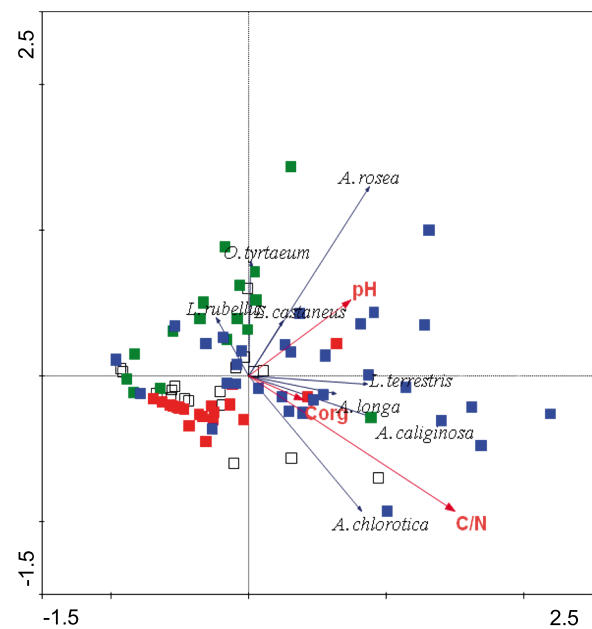
Figure 9. Principal component analysis discerning different crop habitat types, based on abundance of 13 earthworm taxa determined to species level. Green – habitat type 33.01, red – 33.03, blue – 33.04, white – 33 (not assignable to level two). Length of gradient from detrended correspondence analysis = 3.3, first axis = 42.5%, second axis = 13.4% of variance. Only species with a contribution of >15% to the ordination are displayed.
