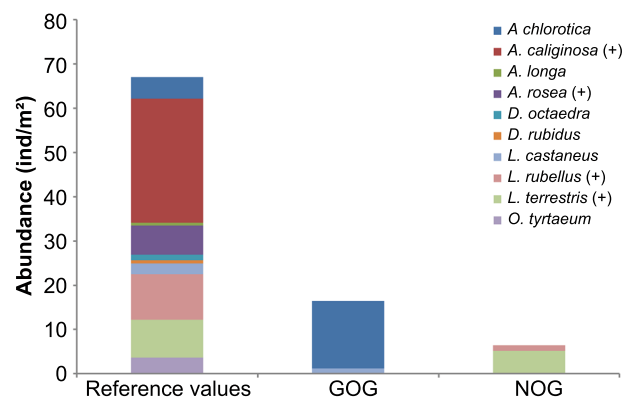
Figure 10. Reference values for uncontaminated grassland sites: mean abundance (ind./m 2 ) of earthworm species (+ = occurrence at >50% of all sites; see Tab. 2) and comparison with abundance and species composition of contaminated sites Gorleben (GOG) and Nordenham (NOG) in Lower-Saxony, Germany.
